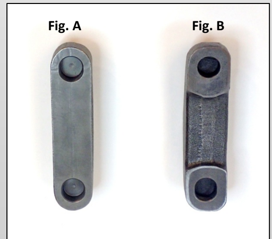
M-3633731 Valve Bridge (Fig. A)
