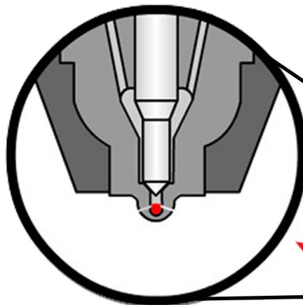
Standard Nozzle
