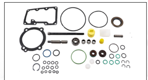
M-3190677RK* - C7/C9 Fuel Pump Kit*
